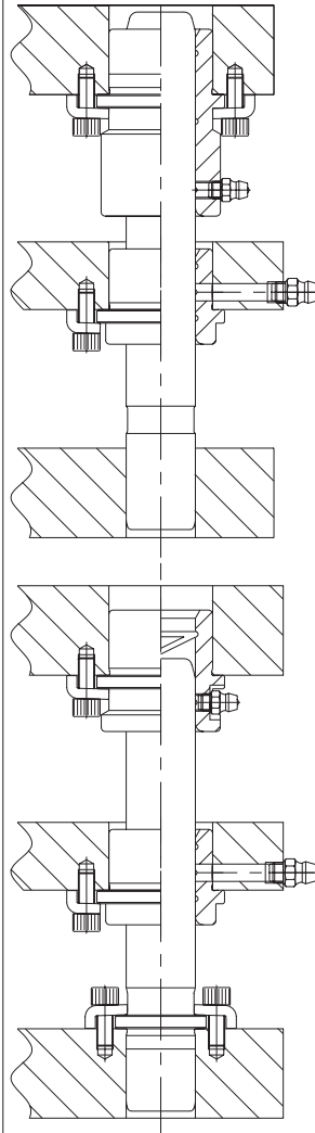
DEMOUNTABLE GUIDE POSTS
